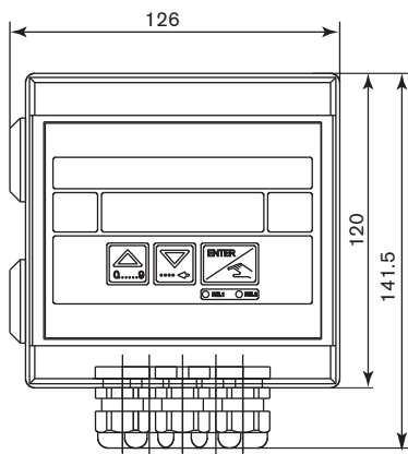
Wall-mounted version
