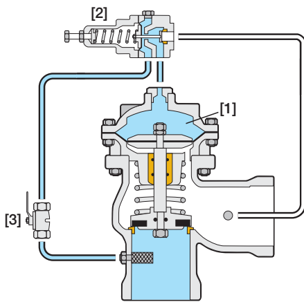
Valve Closed (system pressure is below setting)
