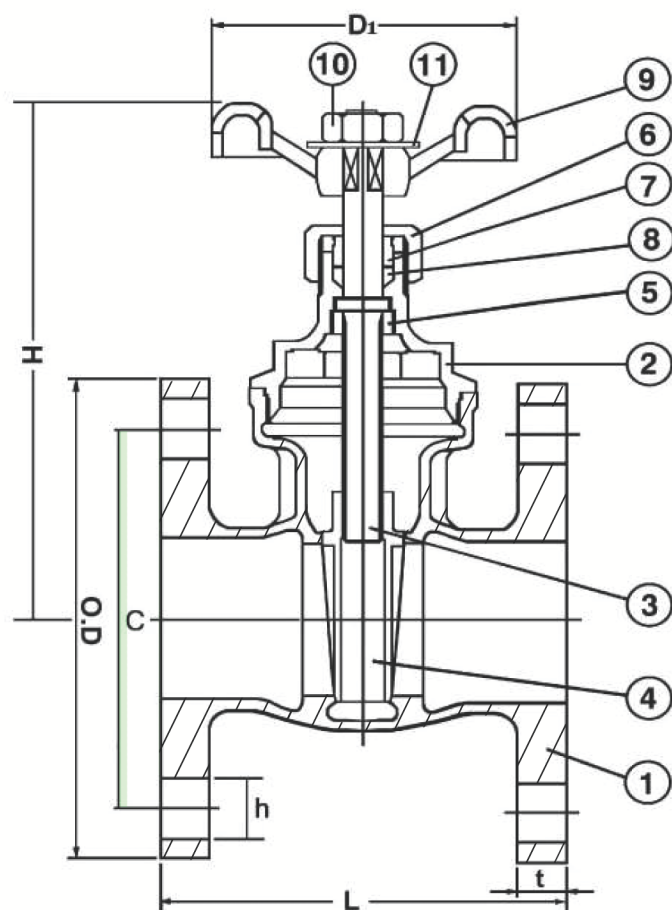
DIMENSION (mm)
